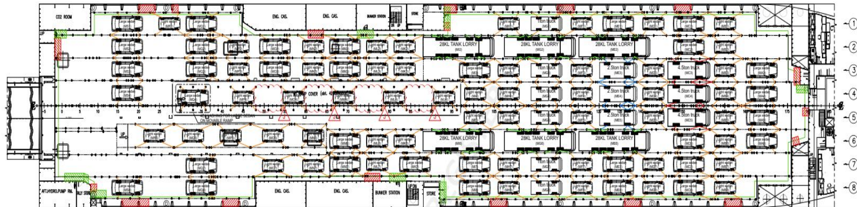
No.1 DECK (TANK TOP)
