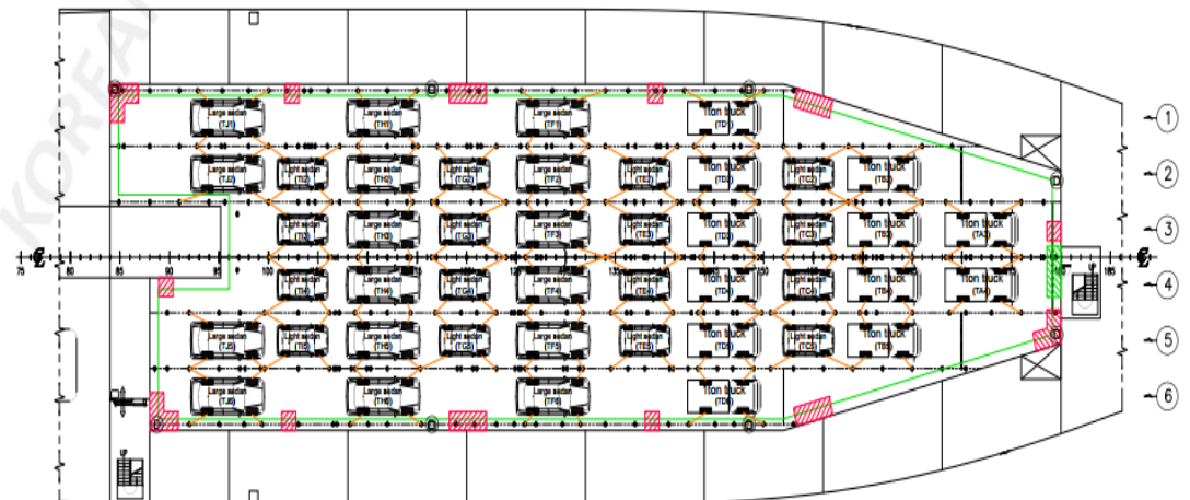
No.1 DECK(TANK TOP)
