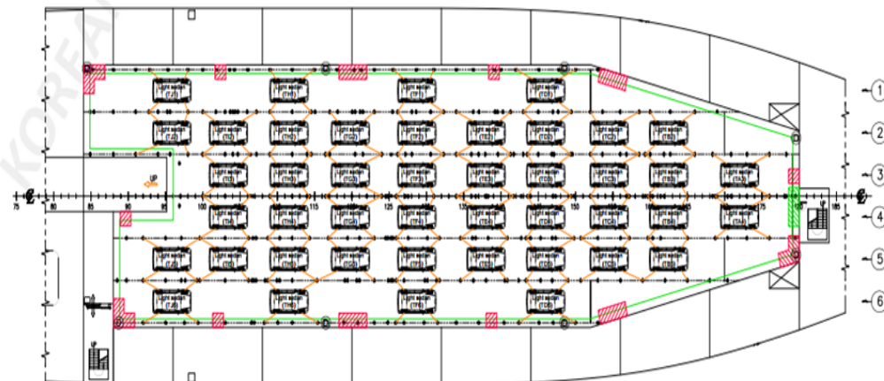
No.1 DECK(TANK TOP)
